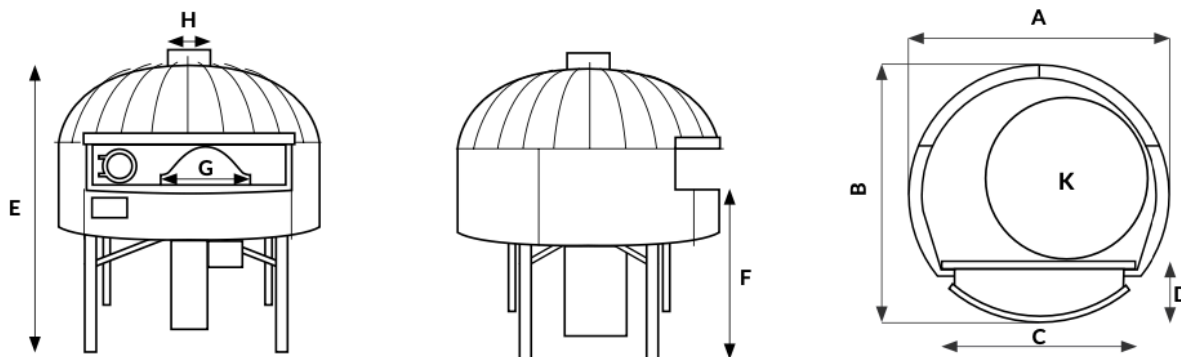
A Oven Width | B Oven Depth | C Frontal Width | D Frontal Depth | E Oven Height F Height From The Floor | G Oven Door Width | H Exhaust Diameter
